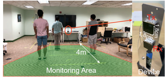
Fig. 11. Experimental scenario and device setup.
