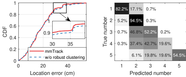
Fig. 14. Benefits of robust clustering, which improves (b) the target detection accuracy significantly, yet only yields marginal gains in (a) location accuracy.
