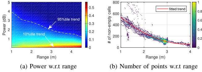
Fig. 4. Measurements on the near-far effect and the effects of weighted resampling. Colors indicate the data density.
