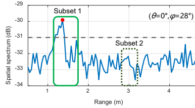
Fig. 7. The spatial spectrum in a specific direction ( \theta = 0^\circ, \phi = 28^\circ ) in which only one subject presents in the range of Subset 1.
