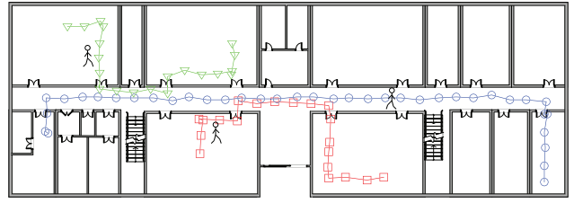
Figure 4: Moving paths.
