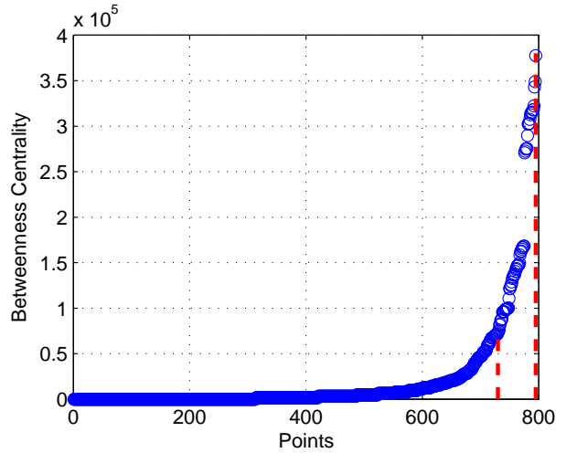
Figure 11: Betweenness distribution.
